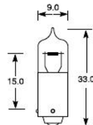
H21W BAY9s
