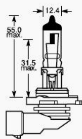
H10 PY20d
