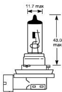
H8 PGJ19-1
