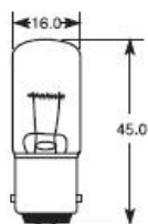
BA15d
