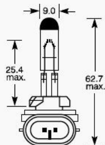
H27W/2 PGJ13
